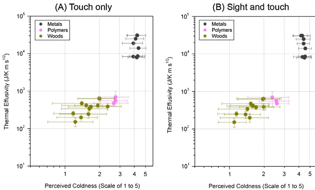
Fig. 4. A plot of the thermal effusivity versus perceived coldness for the 23 materials: (A) data collected under the unsighted condition (participants were blindfolded); (B) data was collected under the sighted condition . The data is categorised by material class, each data point represents the response averaged for all participants.
